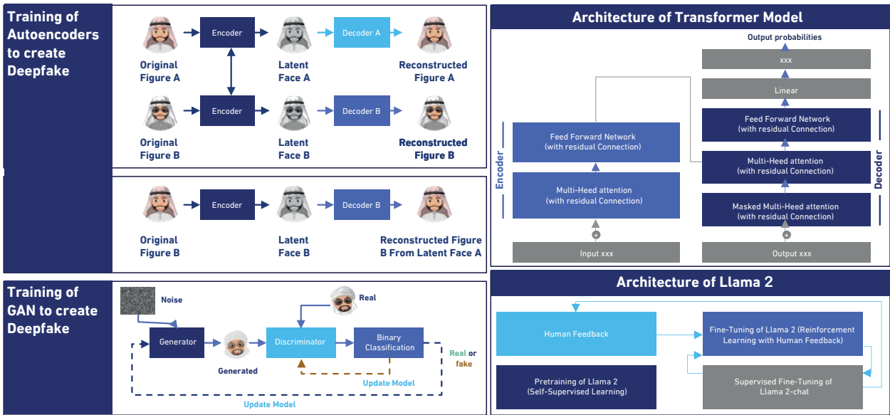
Figure 2: Processes for generating deepfakes
